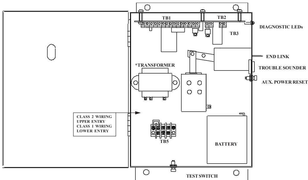
MODEL LM90-B2 INSIDE VIEW
