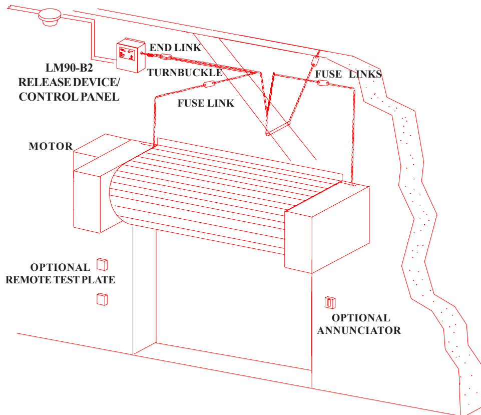
* TYPICAL INSTALLATION
